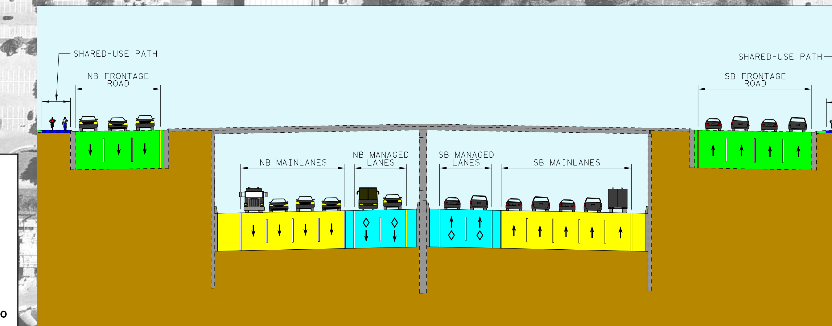
SECTION O-O
