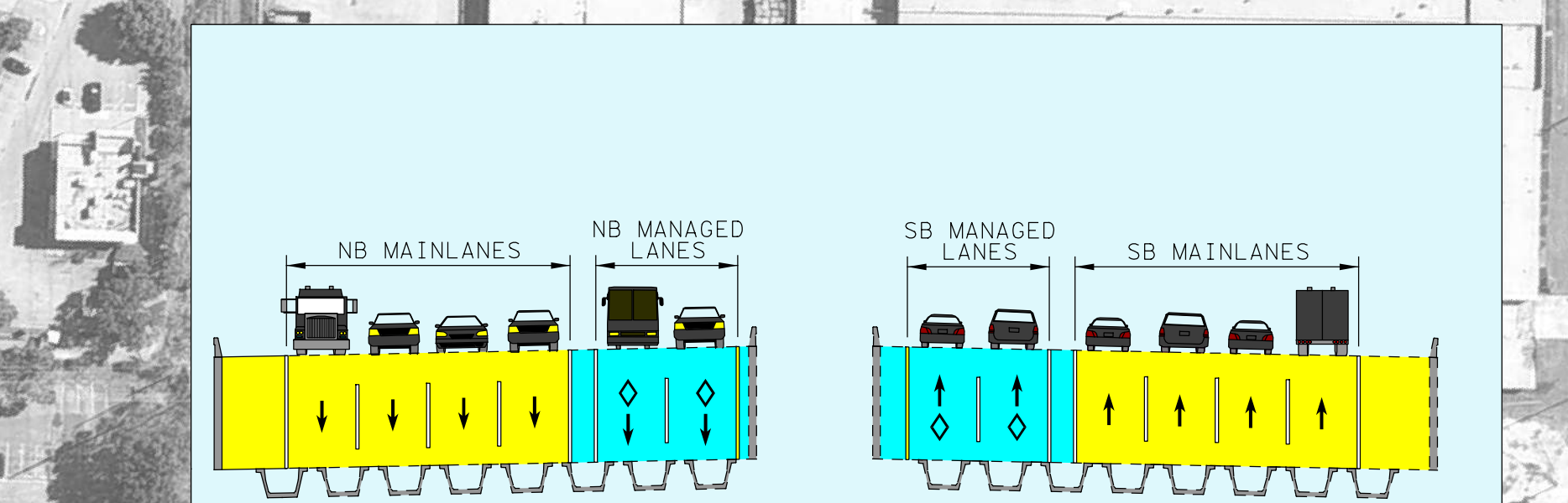
SECTION P-P
