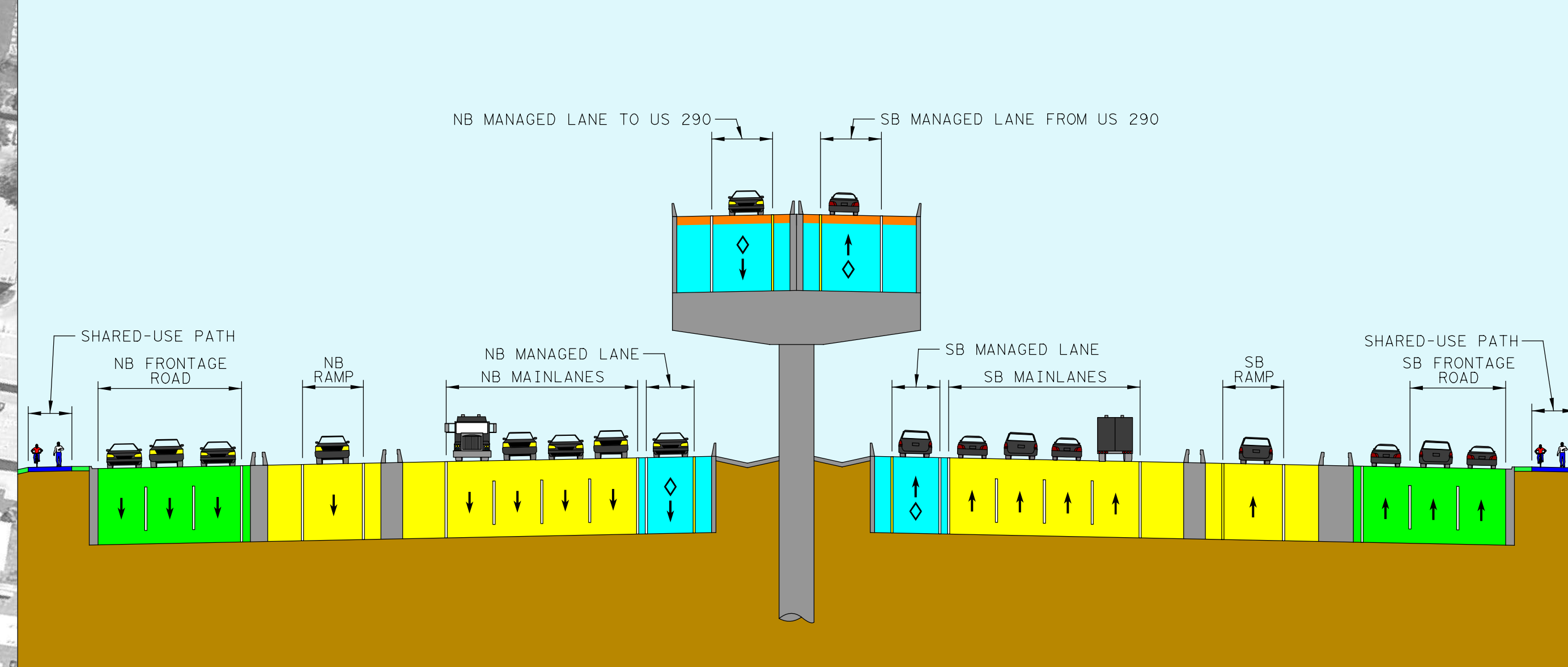
SECTION B-B
